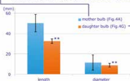
Fig.5. Sizes (mm) of mother and daughter bulbs mean \pm S.D. Welch's t-test (1%) n=94
